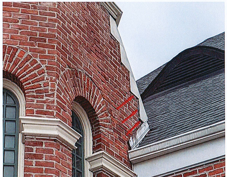
Photo 3 Showing sheet metal cap on lower with large gaps in the mortar joints where the caps are embedded into the masonry. Large open gaps will be repointed and all joints at the embedment areas will receive backer rod and silicone joint sealant.
